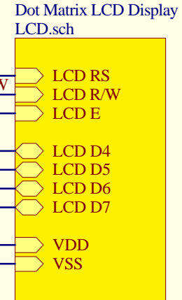
Dot Matrix LCD Display (HD44780 compatible)
